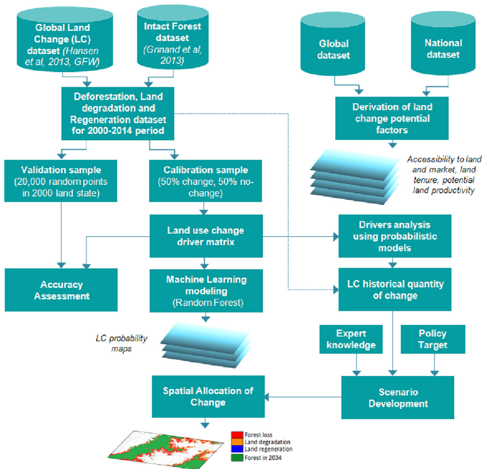
FIGURE 2 Work flow diagram of the different steps carried out in this study [Colour figure can be viewed at wileyonlinelibrary.com ]
