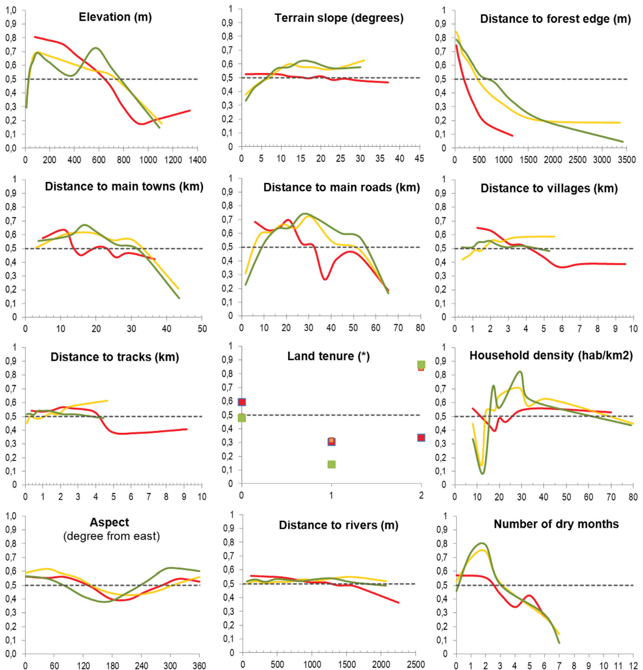
FIGURE 4 Probability distribution of deforestation (red line), land degradation (orange line), and regeneration (green line) observations. The dashed line represents the 50% probability; values above indicates high probability of land change; values below indicates low probability of land change. * indicates land tenure factor. 0 = no protected areas 1 = National park of Andohahela, 2 = National Park of Midongy [Colour figure can be viewed at wileyonlinelibrary.com ]
